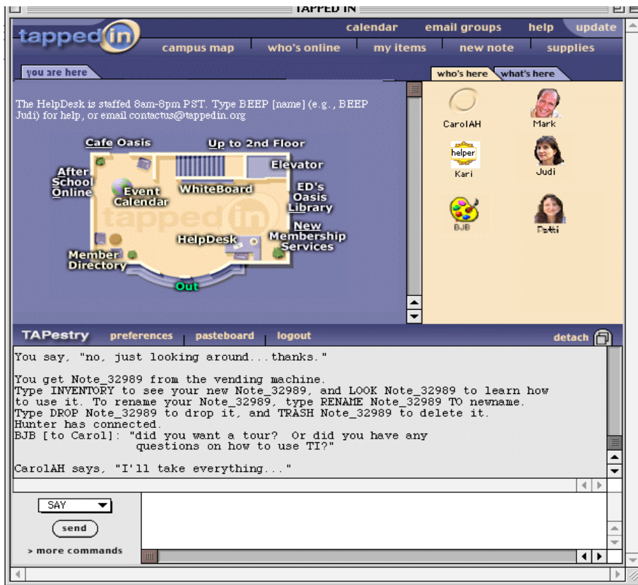
Figure 1. The user interface to the original TAPPED IN testbed system.
