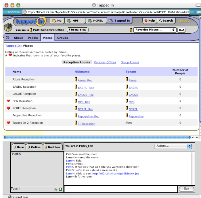
Figure 3. Initial TAPPED IN Version 2 (TI2) interface view of a room, analogous to Figure 1 in the original TAPPED IN. TI2 also uses the metaphor of place, but puts more emphasis on (new) tools and information.
