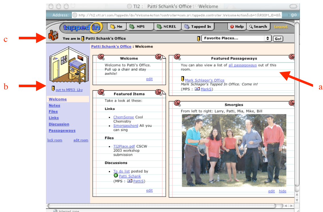
Figure 5. Redesigned TI2 Office with (a) separated Passageways note, (b) new “out” link to the new lobby of the 3 rd floor on which it resides, and (c) icon corresponding to current building (previously, this icon was tied to the customizable room look and feel). (Chat disabled to highlight changes.)
